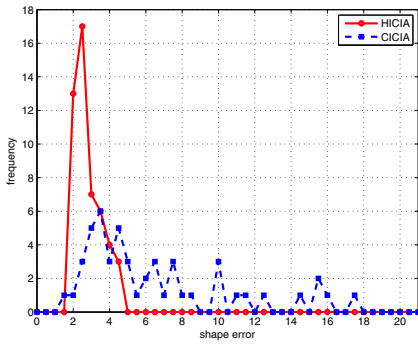
Figure 1. A histogram of the shape errors using the CICA and the HICIA.
