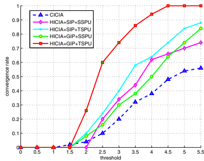
Figure 2. Convergence rates of the different matching methods.
